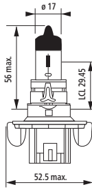
H13 (9008)
