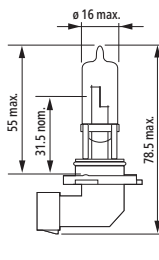
HB3 (9005)
