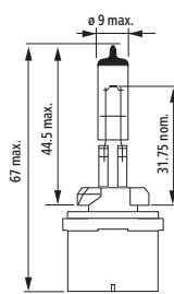
H27W/1 (880)
