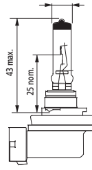
H27W/1 (880)
