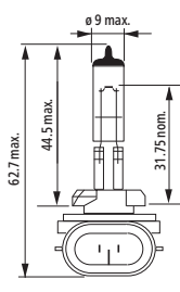
H27W/2 (881)
