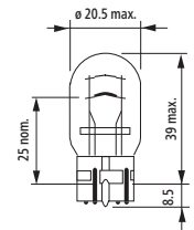
W21/5W
