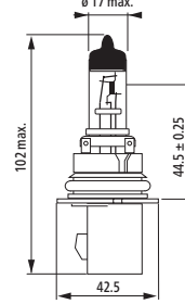
HB5 (9007)
