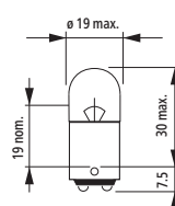
R5W, (BA15d)
